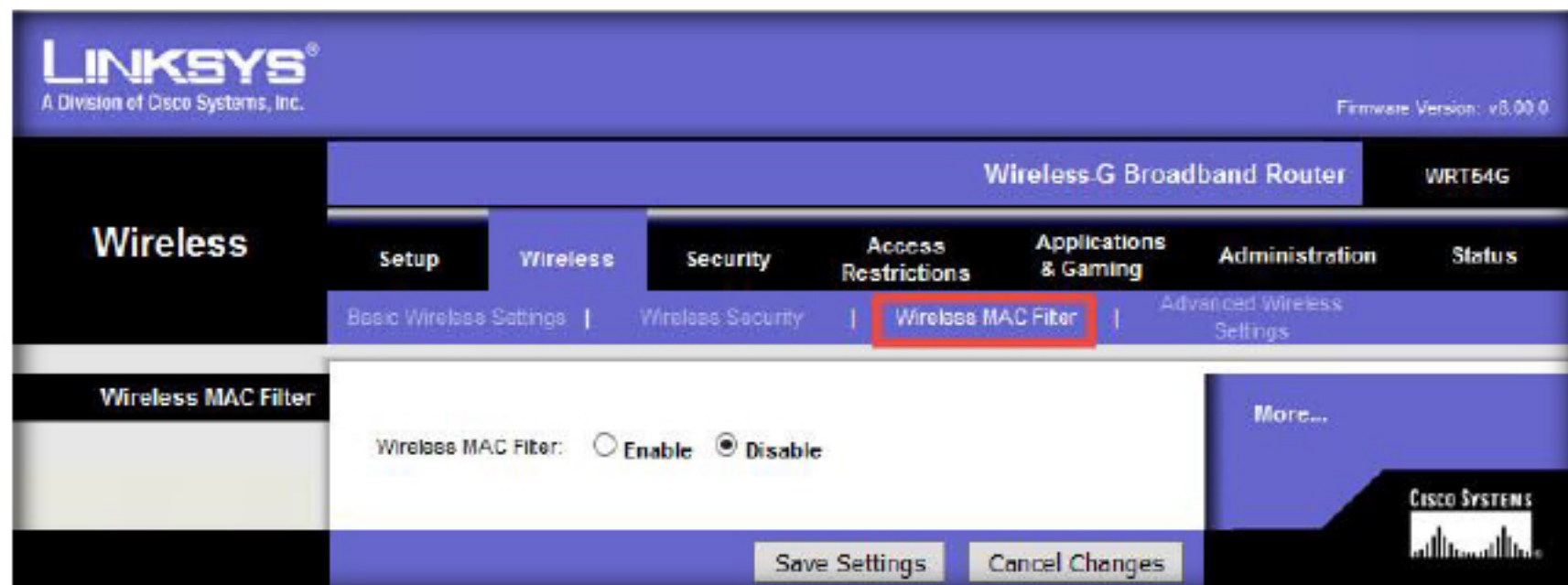
FIGURE 1.36 Wireless MAC filter
