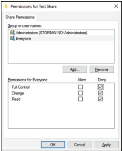
FIGURE 3.13 Setting up permissions on a shared folder
