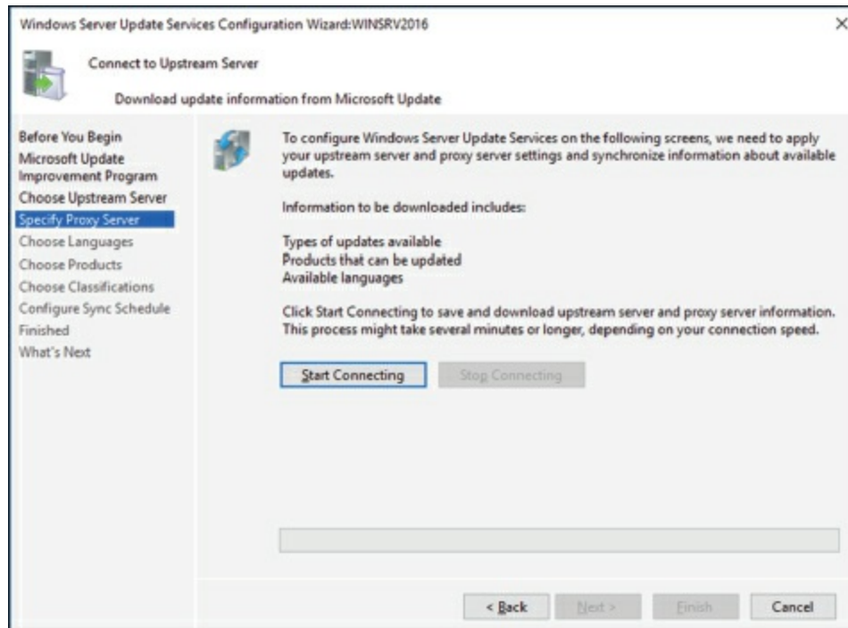
FIGURE 8.13 Connect to Upstream Server
