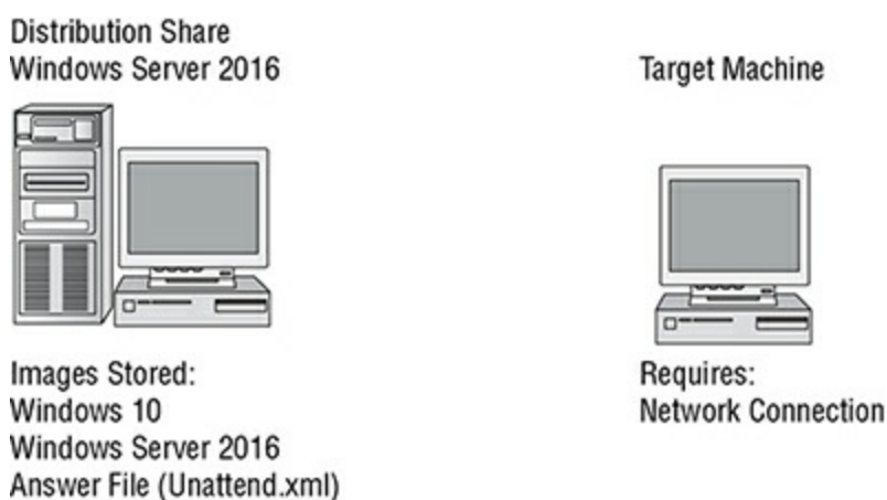
FIGURE 2.12 Unattended installation with distribution share and a target computer
