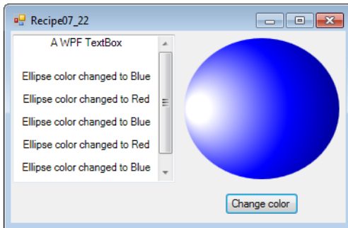
Figure 7-15. Using WPF controls in a Windows Forms form
