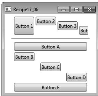
Figure 17-3. Using a StackPanel to control the layout of UI elements
