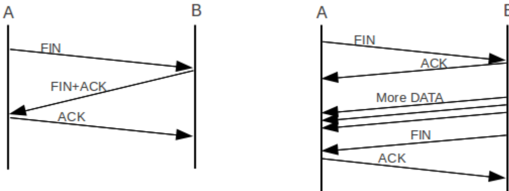
Two TCP close scenarios
