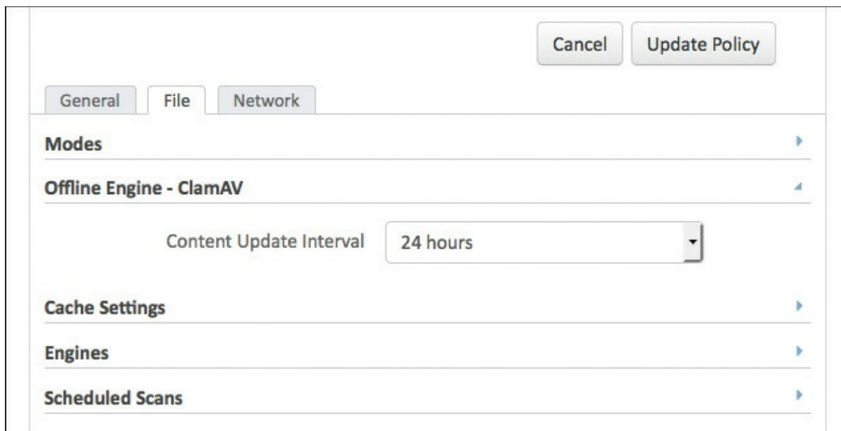
Figure 8-44 Offline Engine—ClamAV
