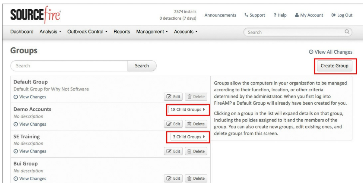
Figure 8-48 Top-Level Groups
