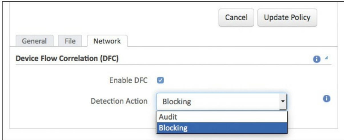
Figure 8-45 Network Tab
