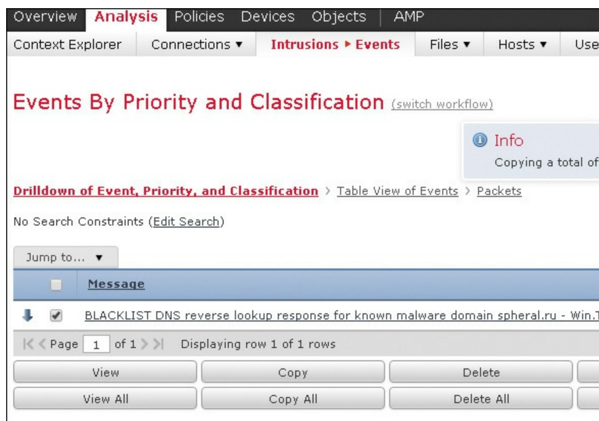
Figure 12-6 Events Workflow
