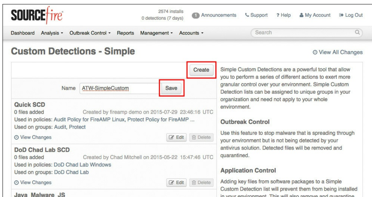
Figure 8-4 Custom Detections—Simple
