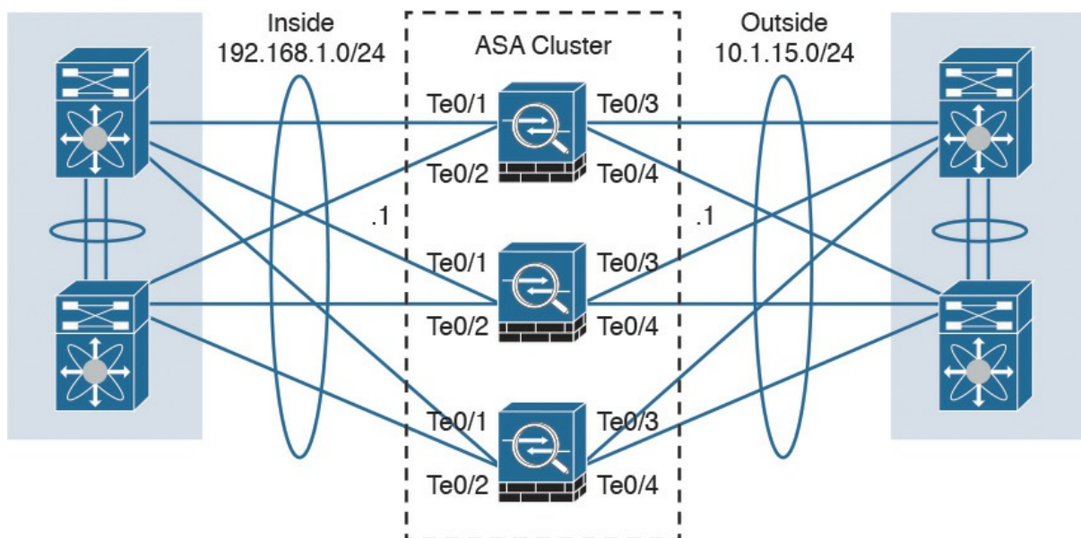
Figure 2-19 Cisco ASA Cluster
