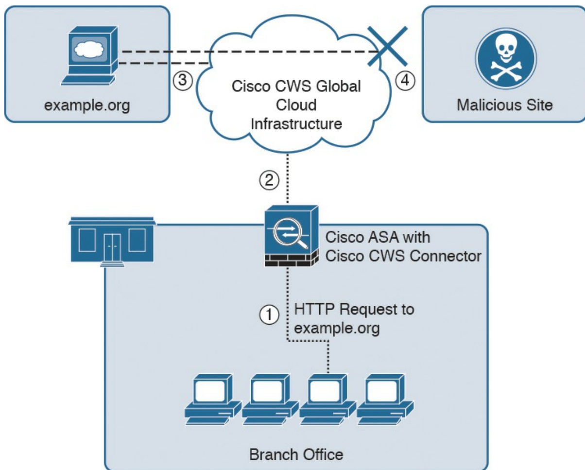
Figure 1-8 Cisco ASA with Cisco CWS Connector Example
