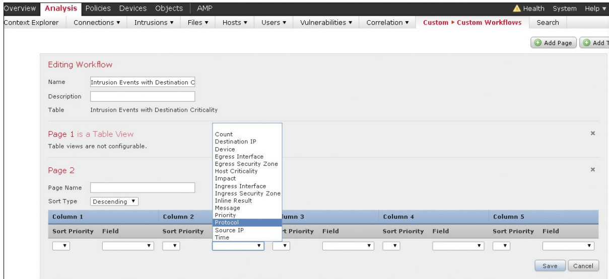
Figure 12-15 Editing a Custom Workflow
