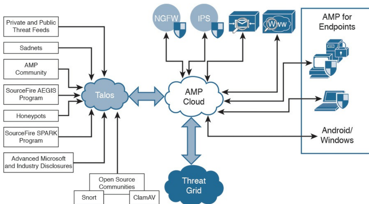
Figure 8-1 AMP Cloud Architecture
