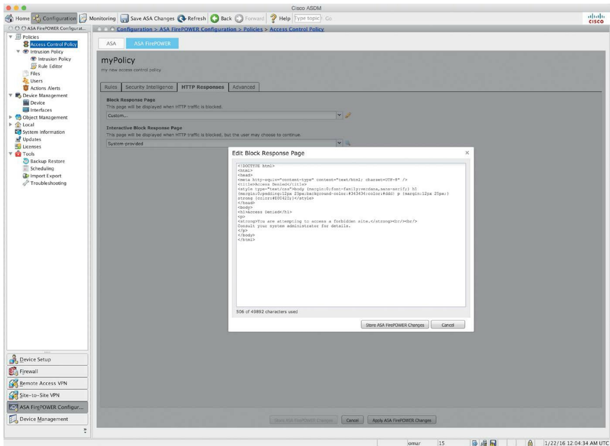
Figure 3-20 Customizing Block Response Pages
