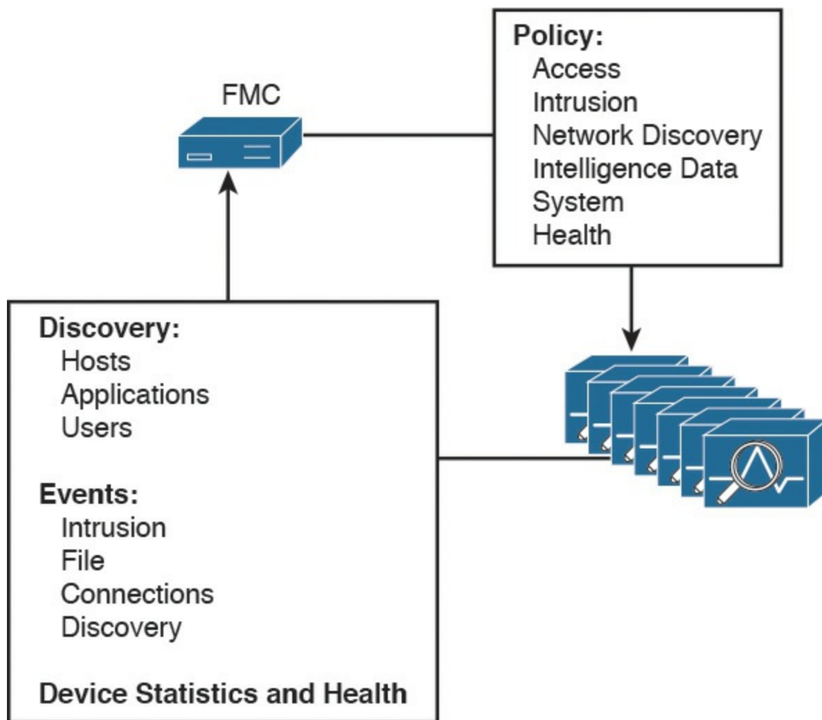
Figure 10-2 FMC Connection Flow with NGIPS Devices
