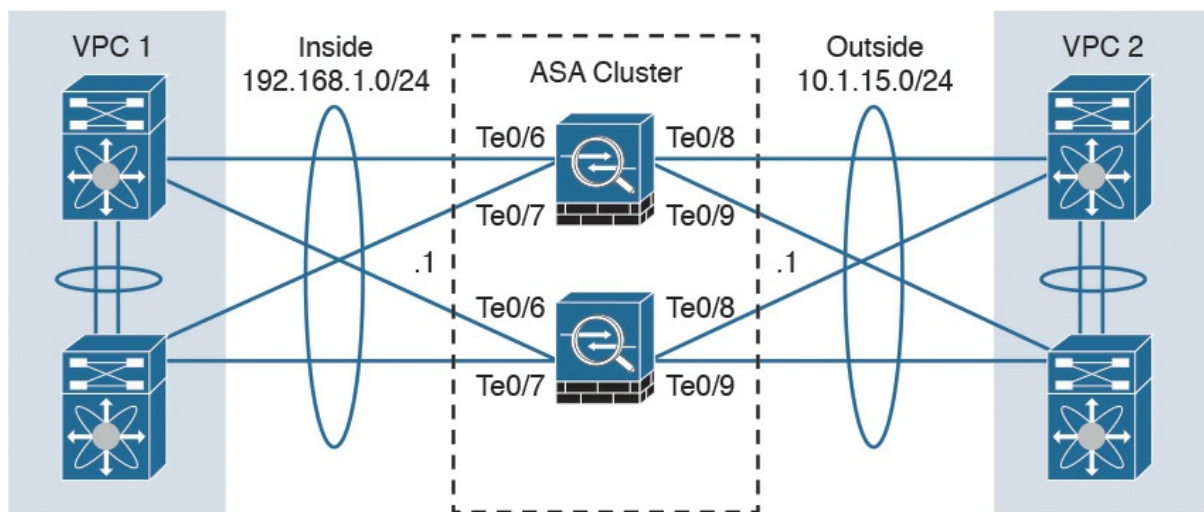
Figure 2-20 Cisco ASA Cluster Configured with Spanned EtherChannel
