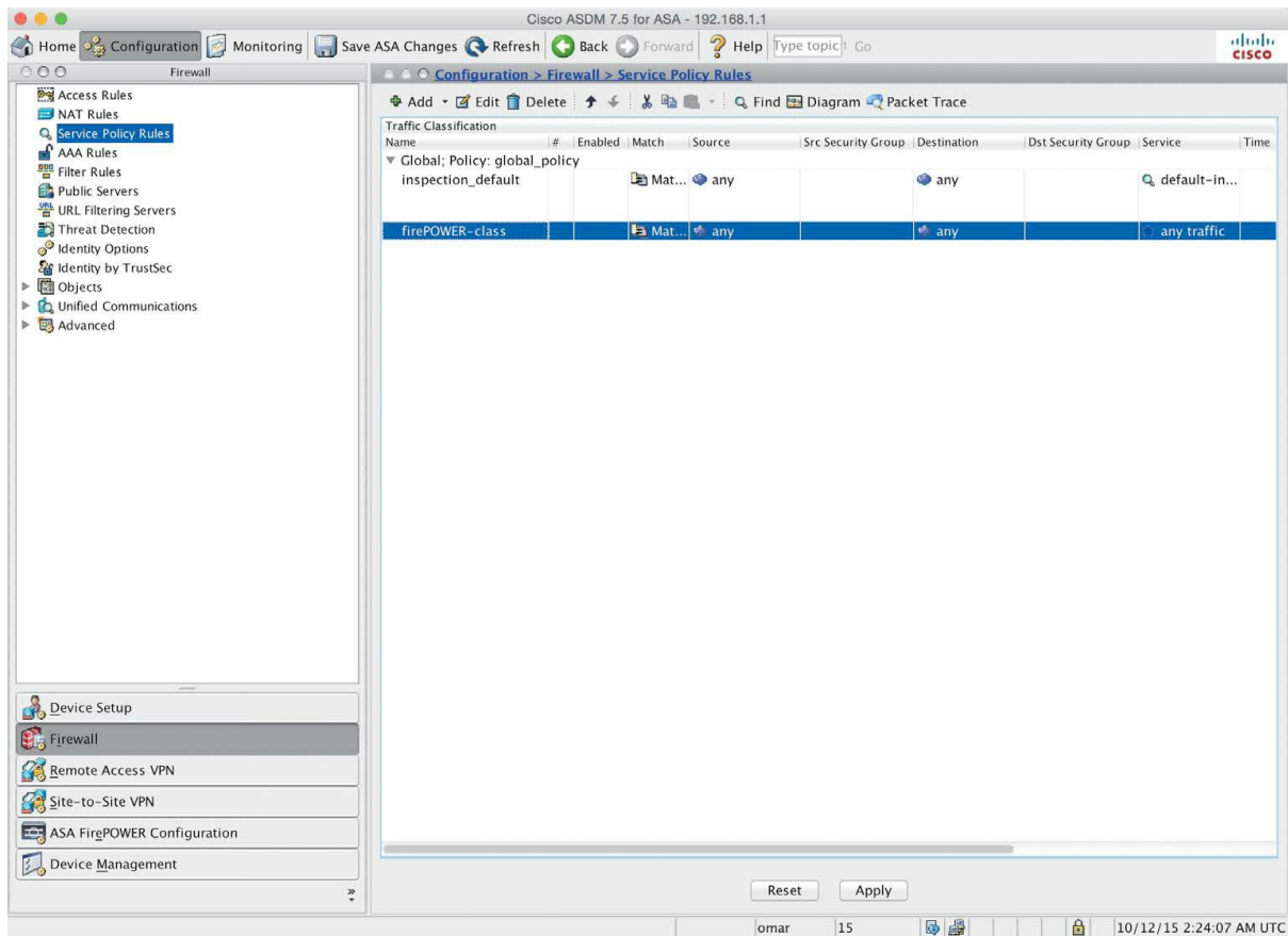
Figure 3-9 The New firePOWER-class Traffic Class
