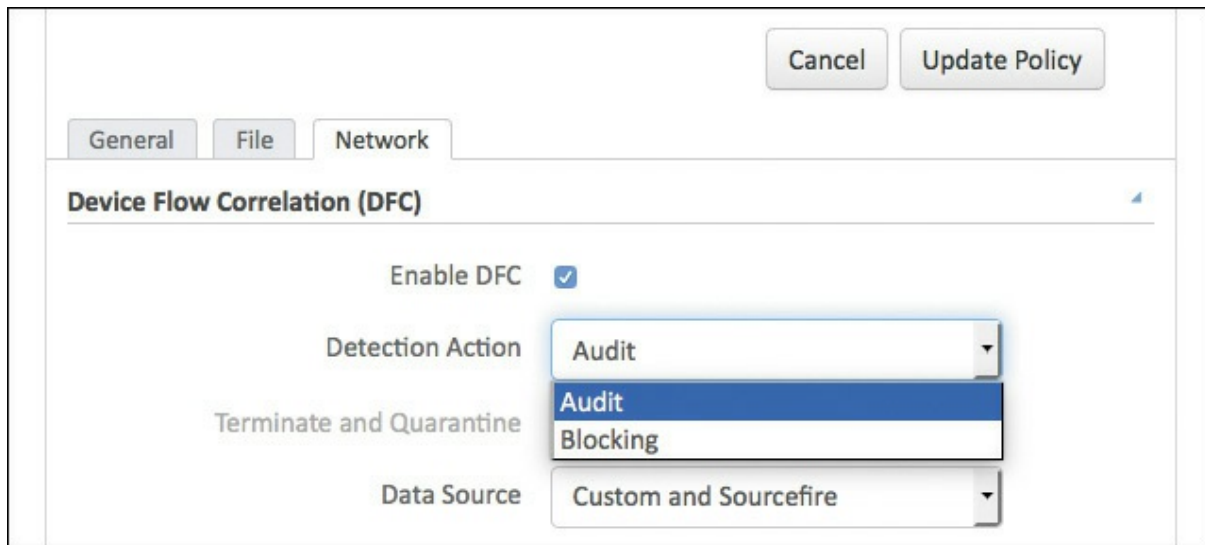
Figure 8-39 Network Tab
