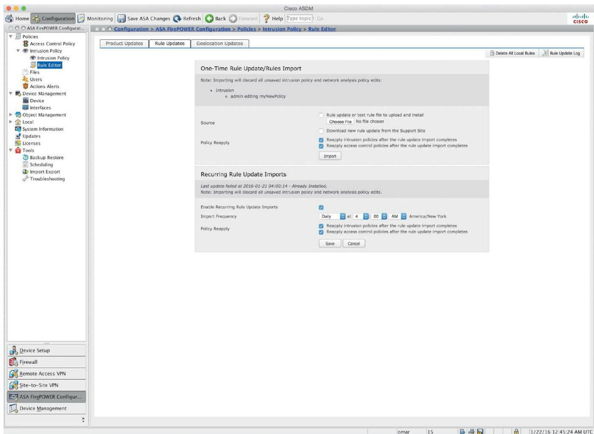
Figure 3-27 Importing Rules
