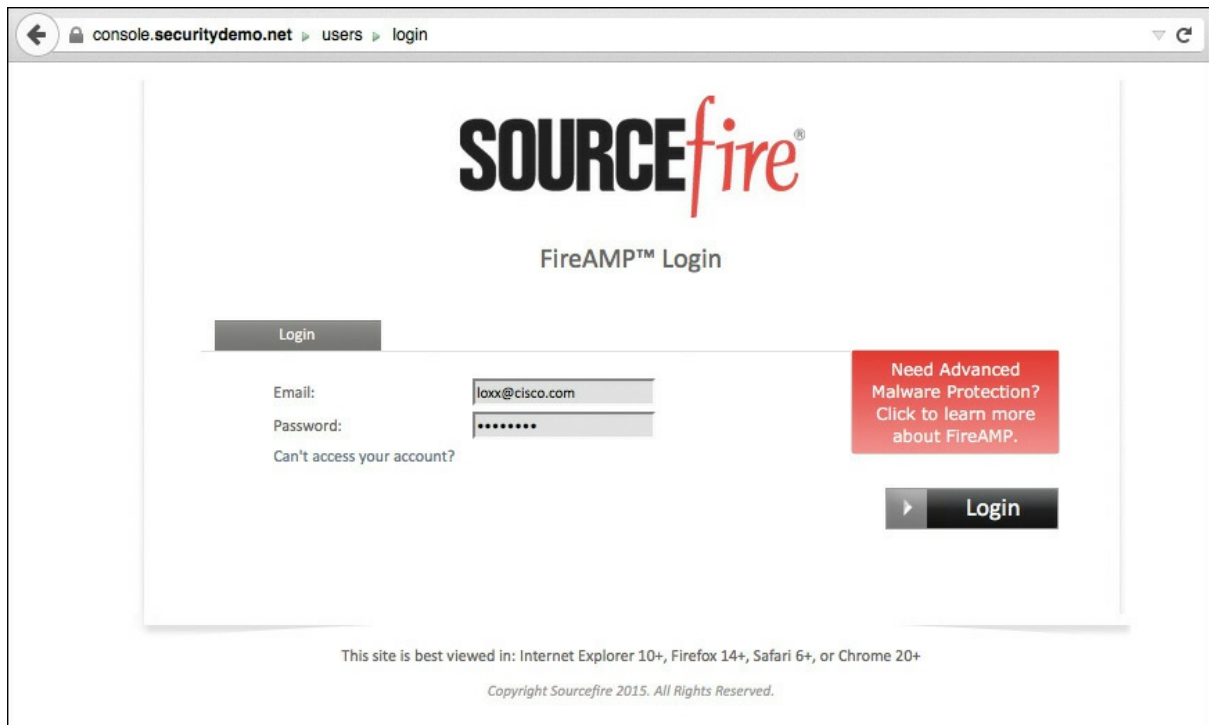
Figure 5-39 Login Screen
