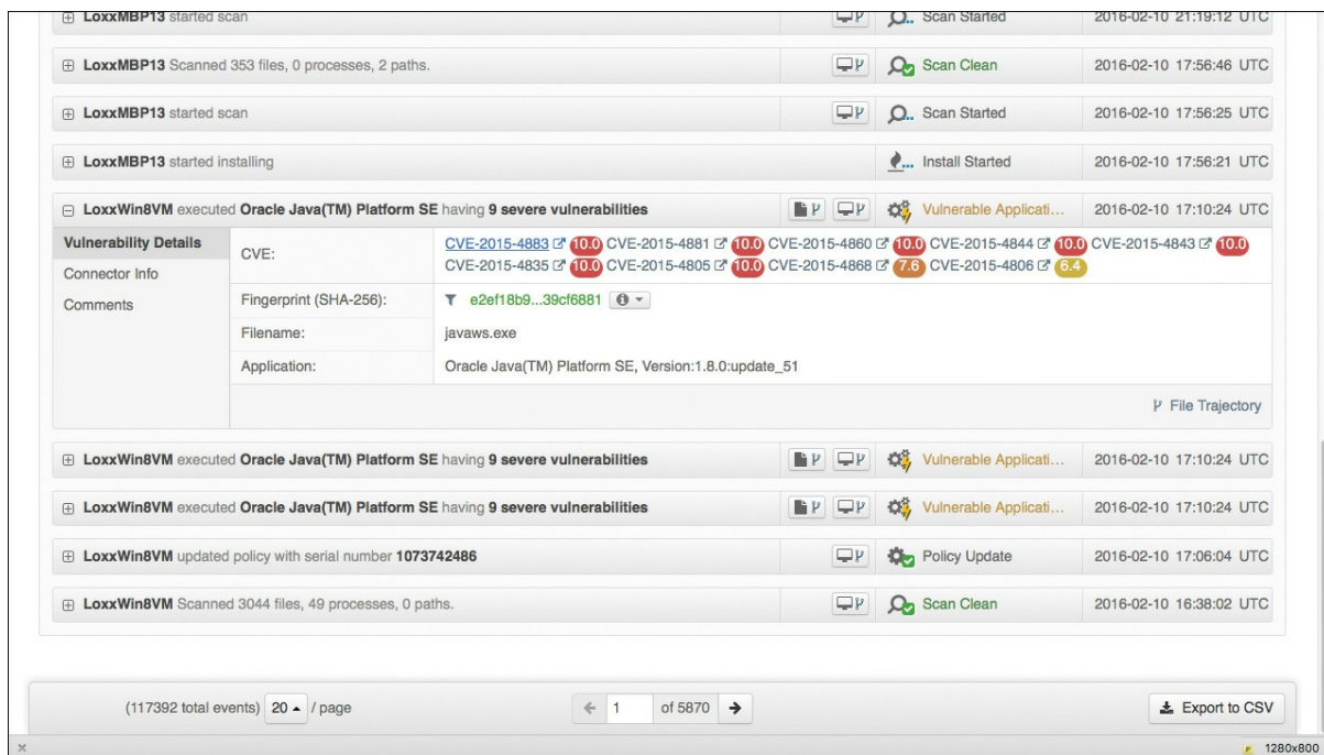
Figure 8-79 Bad Java
