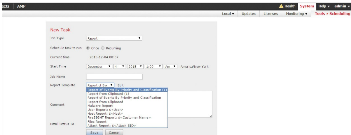
Figure 12-18 Report Scheduling
