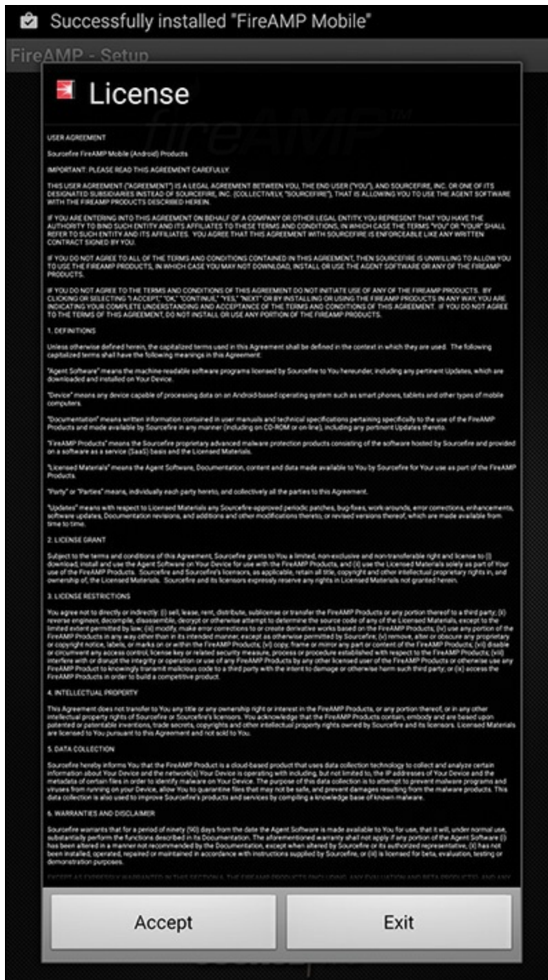
Figure 8-73 License Agreement
