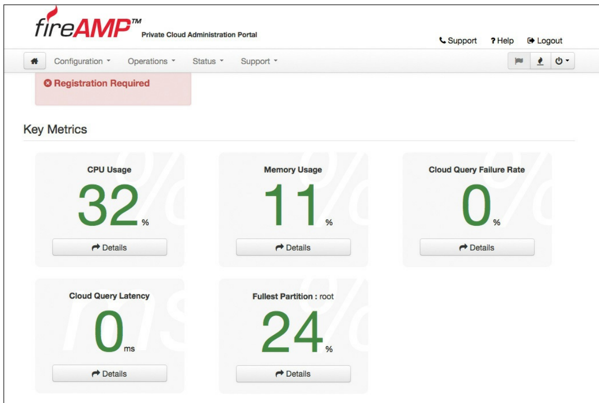
Figure 5-38 Key Metrics
