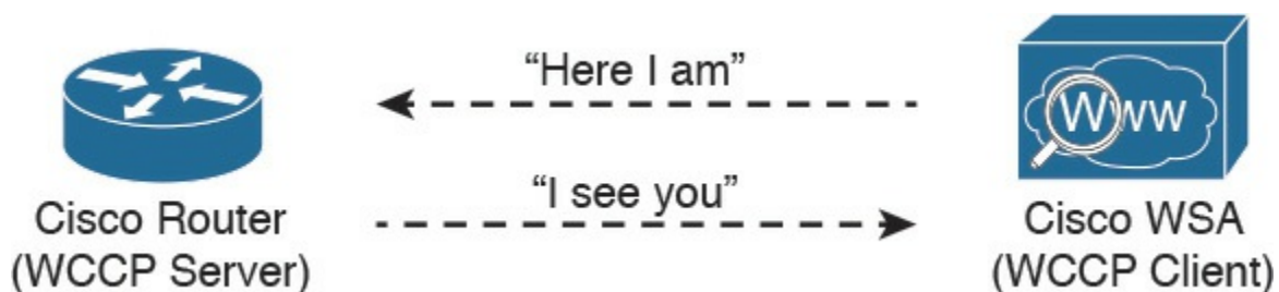
Figure 1-5 WCCP Registration
