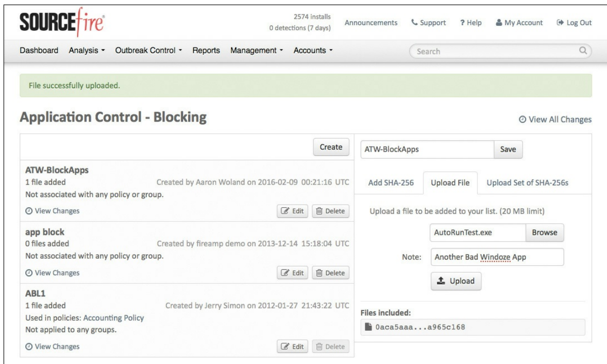
Figure 8-16 Adding Application Hashes to the Blocking List
