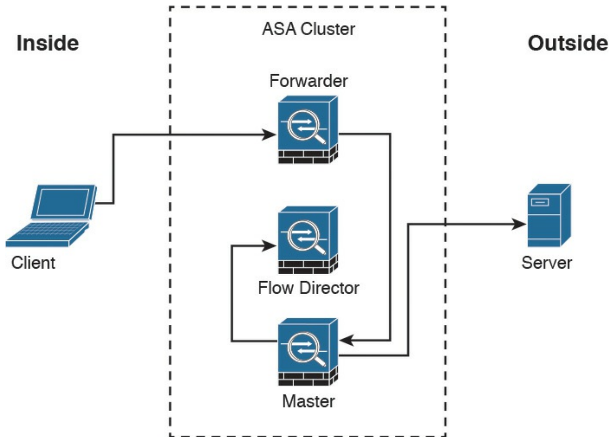
Figure 2-25 Centralized Connections in a Cisco ASA Cluster
