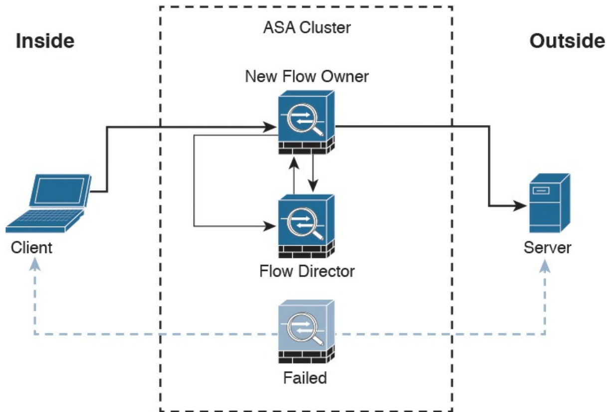
Figure 2-26 Flow Owner Failure
