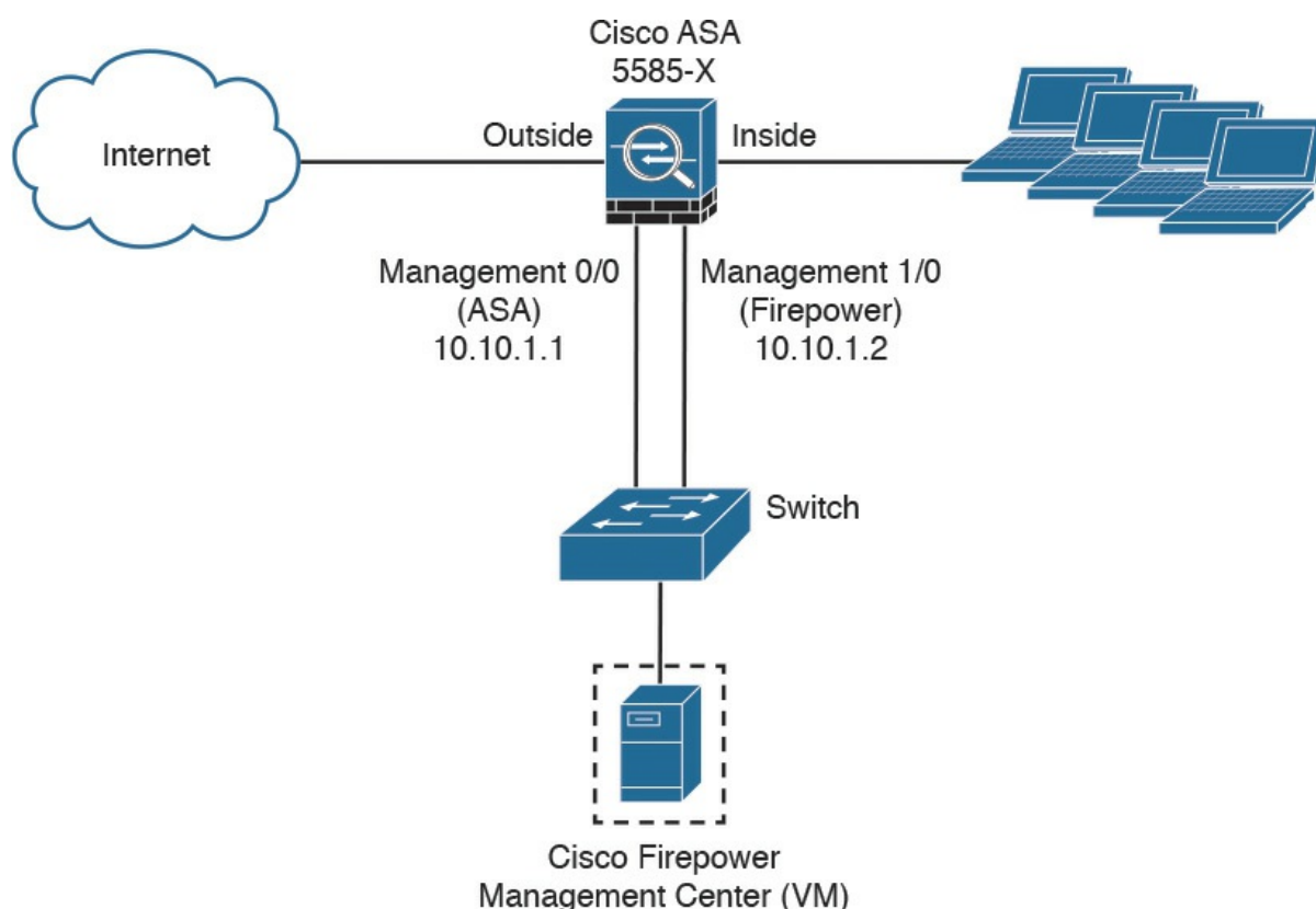
Figure 3-1 Cisco ASA 5585-X Management Interfaces
