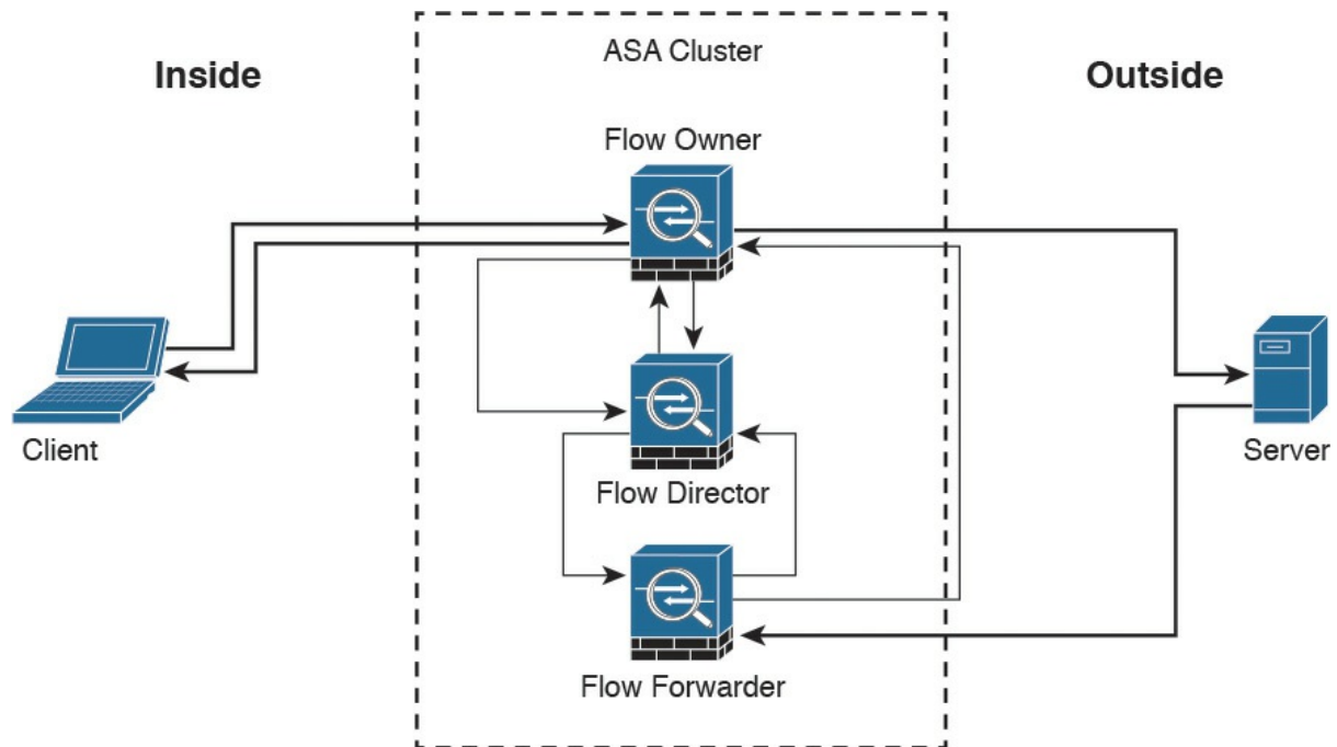
Figure 2-24 A New UDP or Another Pseudo-stateful Connection in a Cisco ASA Cluster
