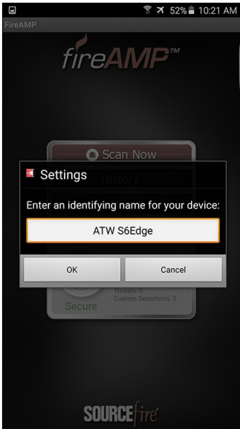
Figure 8-76 Settings
