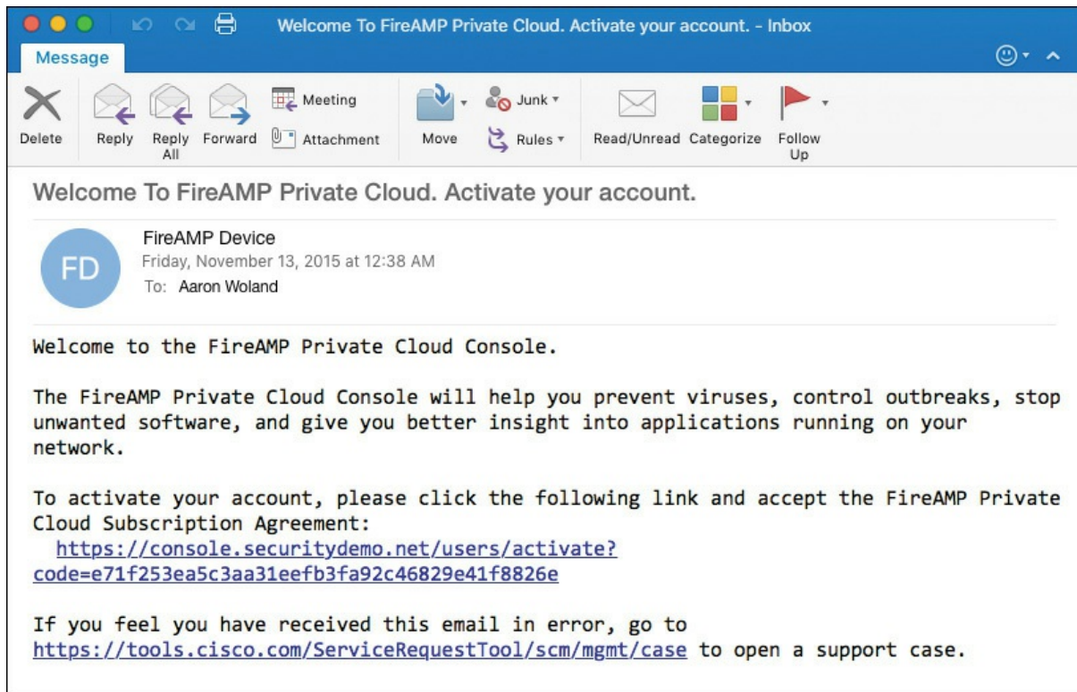
Figure 5-35 Email Notification
