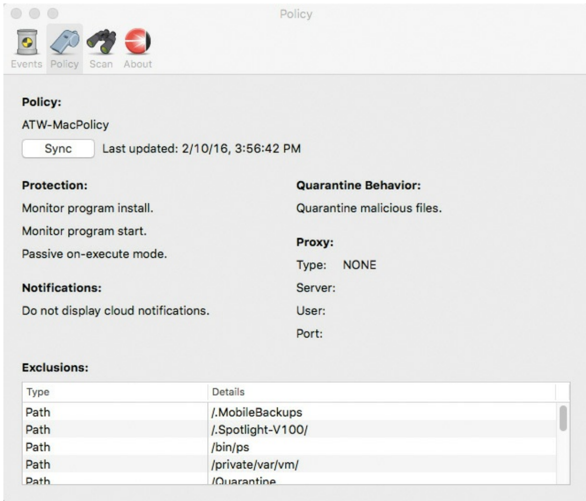
Figure 8-63 Policy Section
