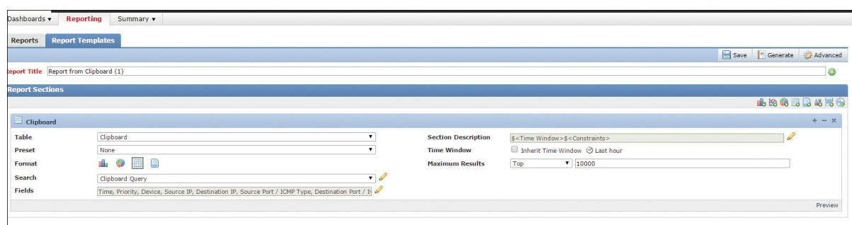
Figure 12-17 Report Template
