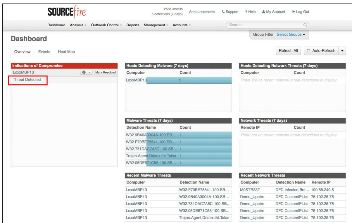
Figure 8-77 Dashboard
