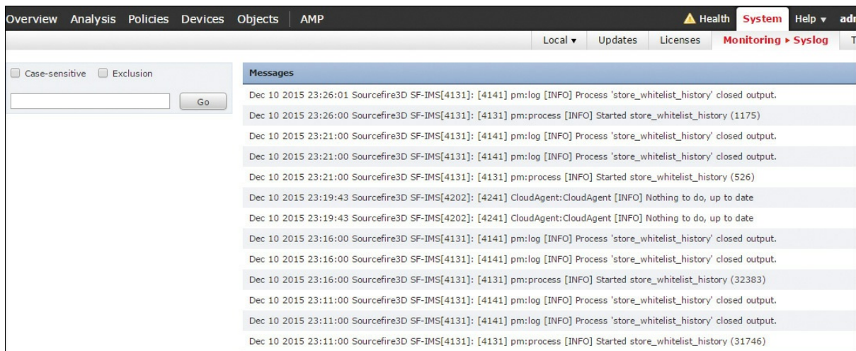
Figure 12-38 Syslogs
