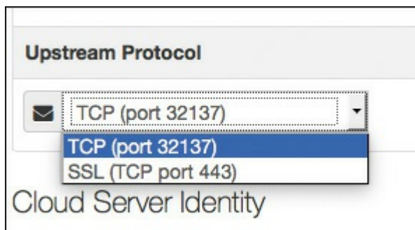
Figure 5-29 Protocol Selection
