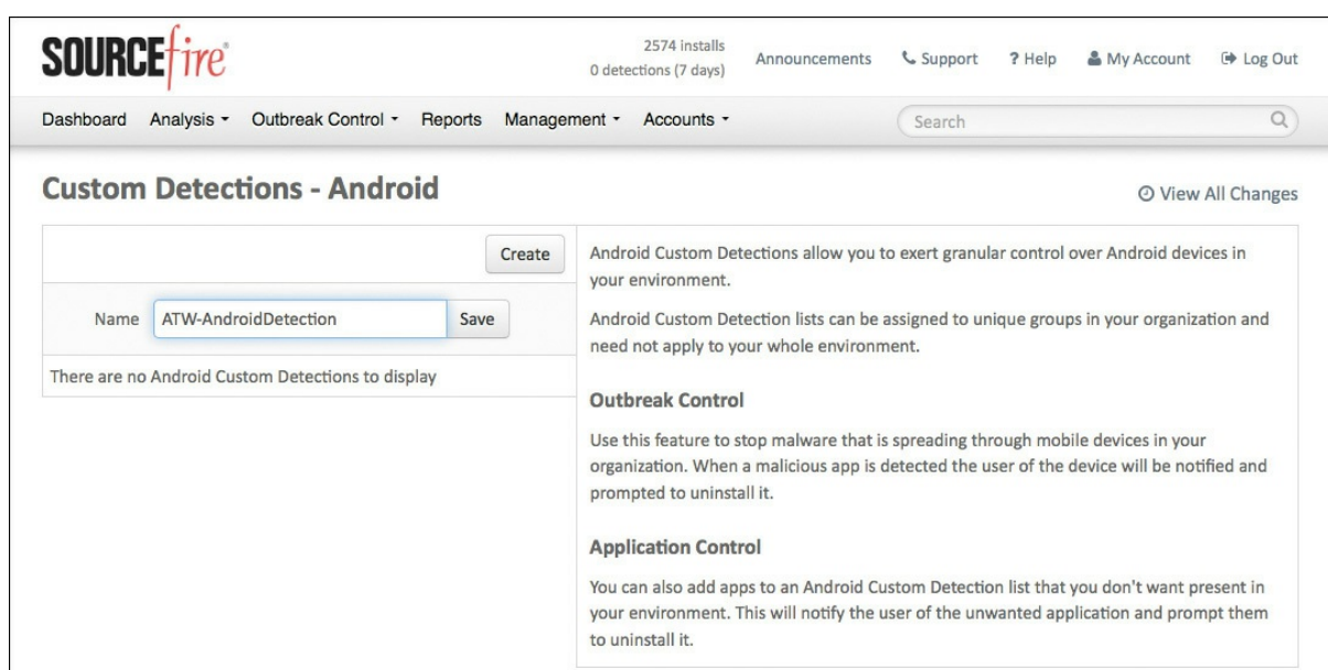
Figure 8-12 Custom Detections—Android
