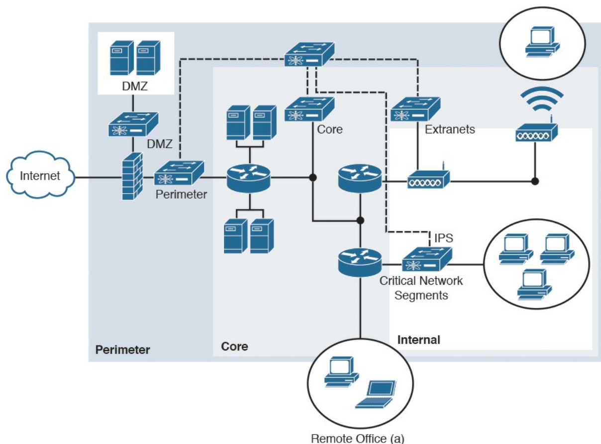
Figure 10-7 NGIPS Deployment Locations
