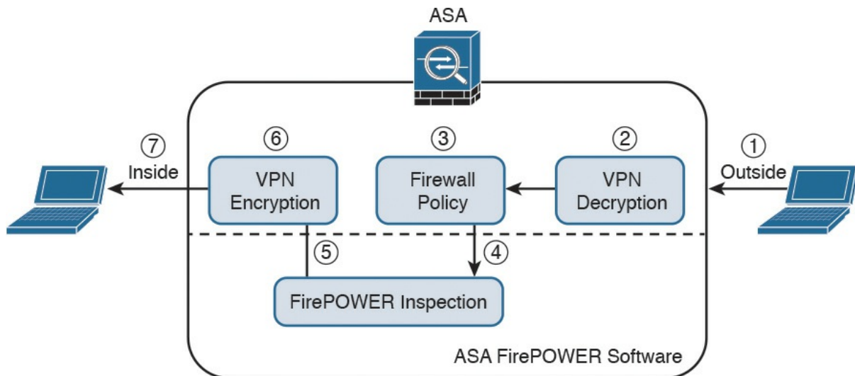
Figure 2-1 Inline Mode
