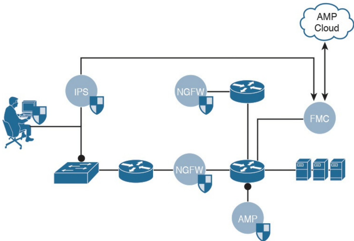
Figure 6-1 AMP Connectors Talking to the DC and Then the Cloud
