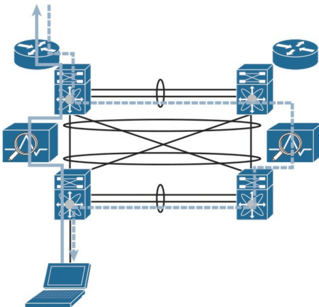
Figure 10-8 Asymmetric Flows in a Redundant Data Center
