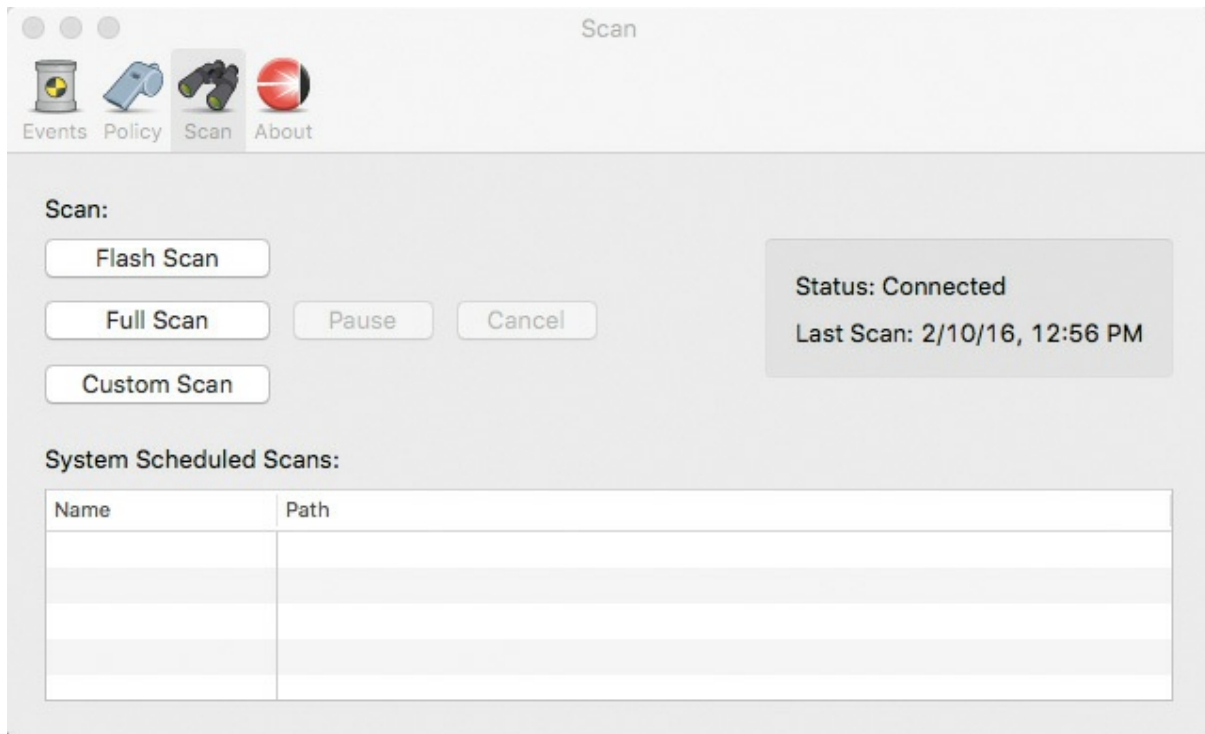
Figure 8-64 Scan Section
