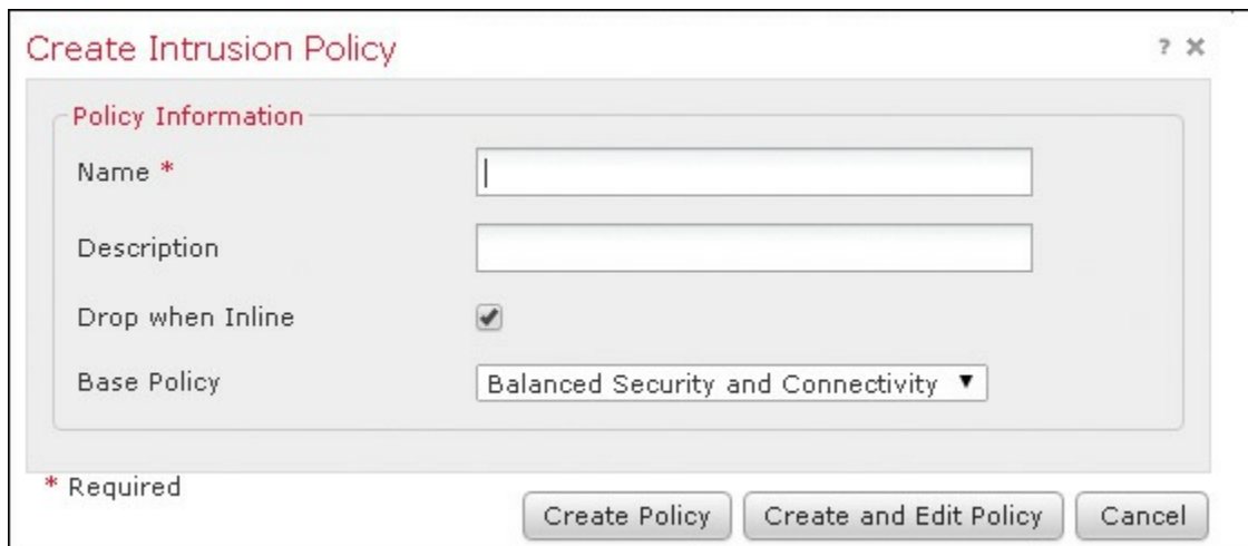
Figure 11-7 New Policy
