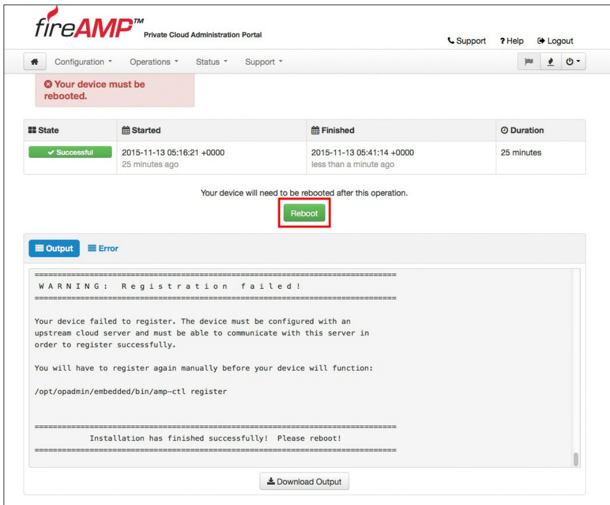
Figure 5-36 Successful Installation
