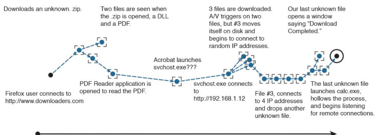
Figure 5-4 Trajectory Illustrated
