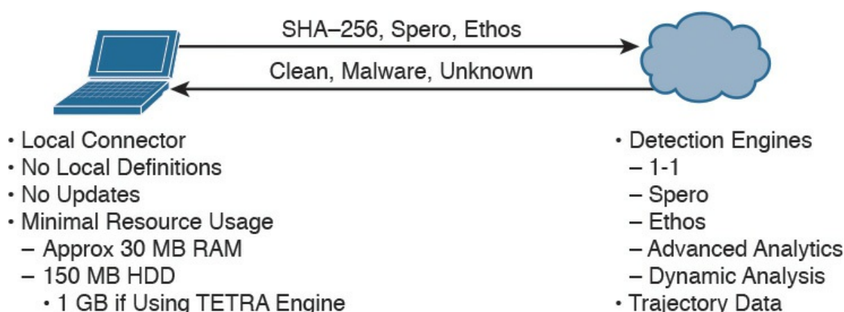
Figure 8-2 AMP for Endpoints Architecture
